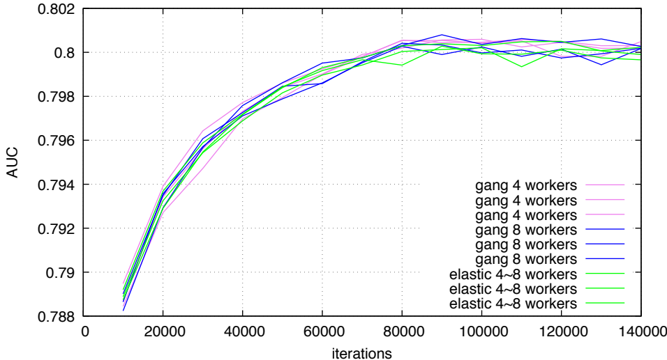
Changing # workers doesn't affect convergence -- wide and deep model
