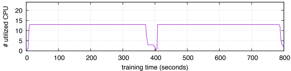
Elastic scheduling -- two jobs overlap and fully use the cluster
